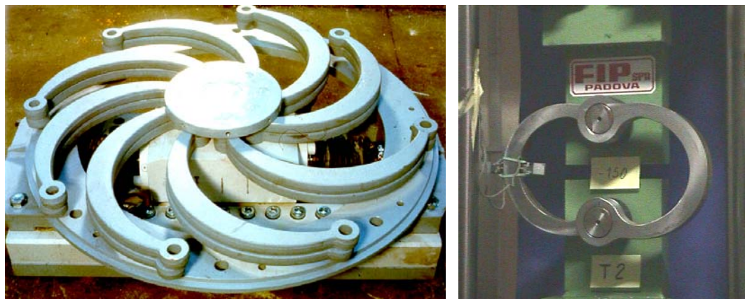
Figure 4 - A multi-directional steel hysteretic damper with crescent moon elements during assembly (left) and two crescent moon elements under testing (right).
