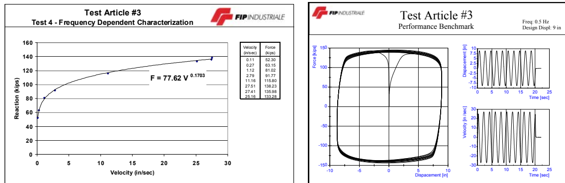
Figure 17 - Force vs. Velocity experimental relationship (left) and typical hysteretic loop of a FIP's fluid viscous damper under sinusoidal excitation (right).
