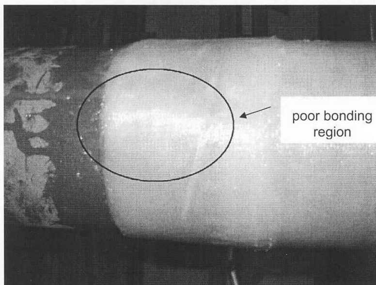
Figure 7: Repaired Pipe - Consecutive Lap Joint
