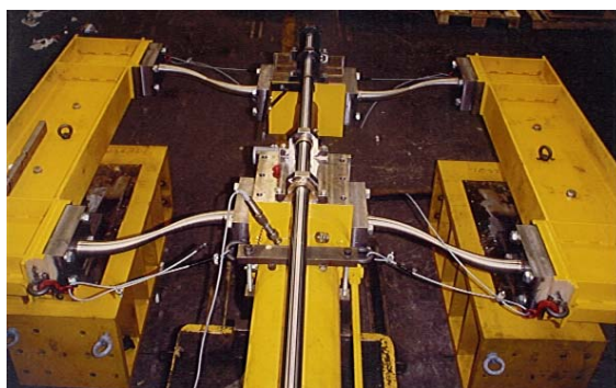
Figure 7 – Double-tapered pins under test and their hysteretic loop.
