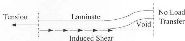
Figure 8:– Load Transfer due to Voids
