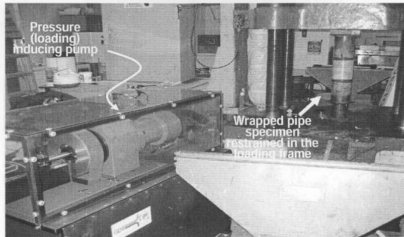
Figure 9: Overall test set up
