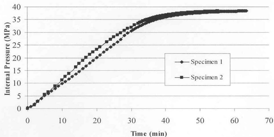
Figure 10: Yielding of Pipe Specimens
