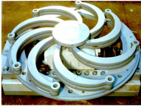
Figure 13 - Isolator with double tapered pin steel hysteresis dissipating element used for the seismic retrofit of the Marquam Bridge, Oregon, USA.
