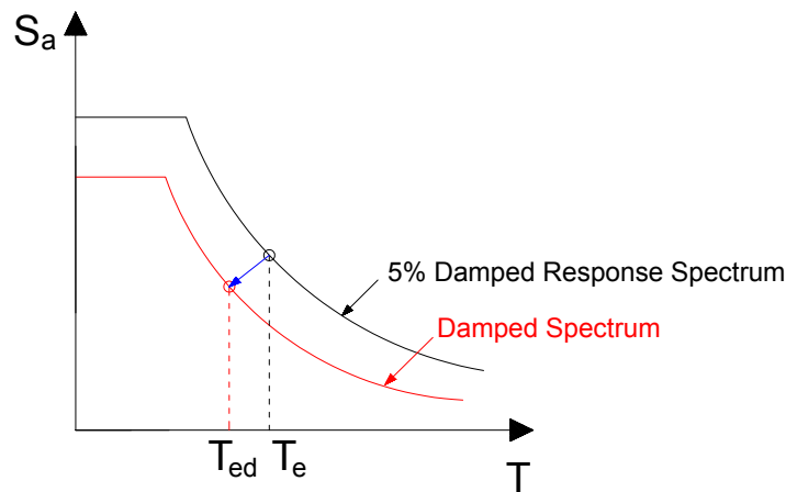
Fig 4: Period Shifting Effect in Spectral Reduction
