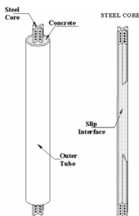
Fig.11. Scheme of a buckling restrained axial damper on the left and its steel core member on the right.
