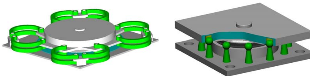
Figure 9 –Examples of sliders with steel hysteretic dissipating elements of the crescent moon type (left) or of the tapered pin type (right).
