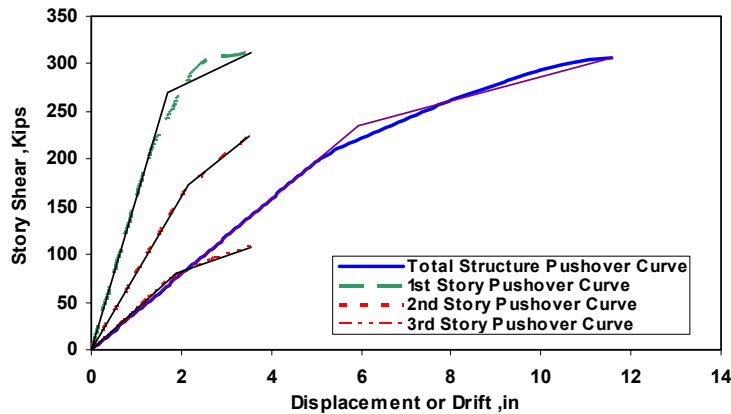
Fig.5: Pushover of each Story and Total Pushover Curve for 1st Mode Lateral Force Pattern with P- \Delta Effect
