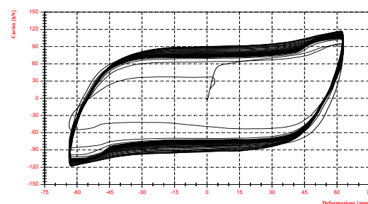
Figure 6 - Tapered pin under test and hysteretic loop.
