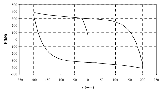
Figure 7 – Double-tapered pins under test and their hysteretic loop.
