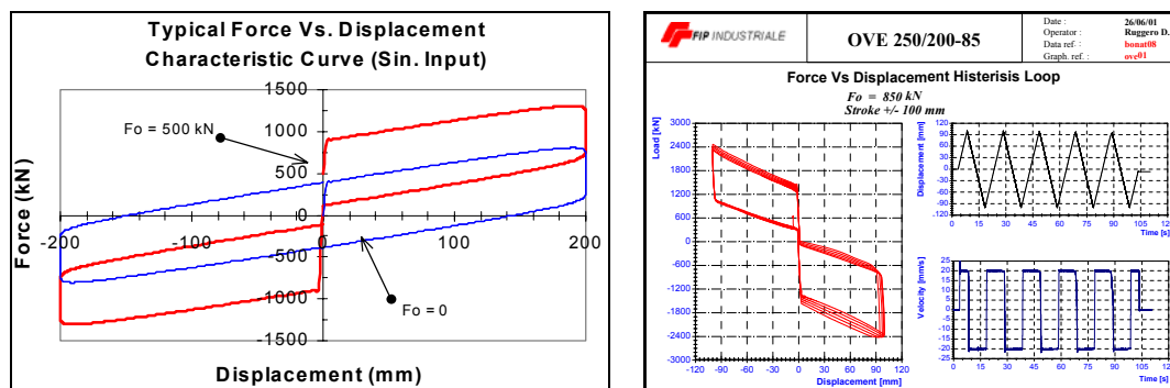
Figure 19 - Typical theoretical and test hysteretic loop of a spring fluid viscous damper.
