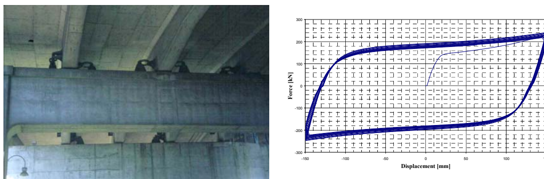
Figure 5 –Steel hysteretic dampers with crescent moon elements as installed in the Granville Bridge (left) and a typical force vs. displacement experimental curve of this type of damper (right).
