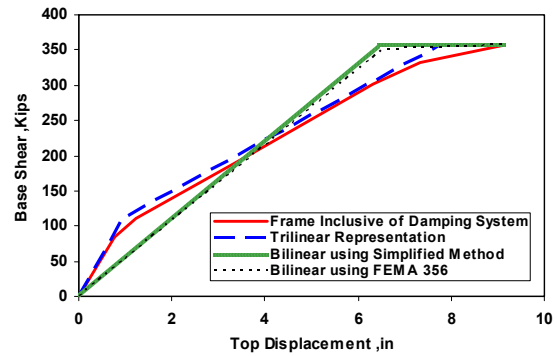
Fig. 7: Bilinear and Trilinear Representation of 3 Story Pushover Curve of the Building with Friction Damping System
