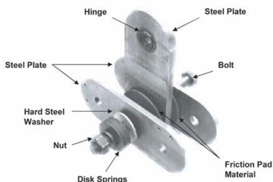
Fig. 1: Components of Friction Damping Device
