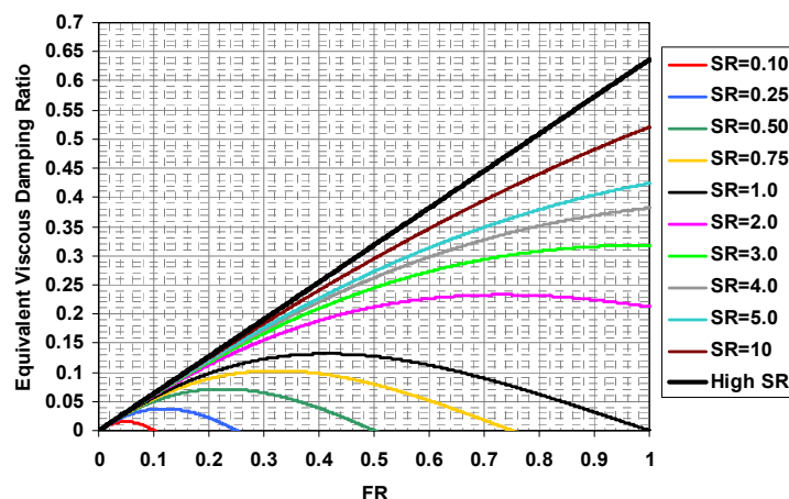
Fig. 3: Equivalent Viscous Damping for Dual System
