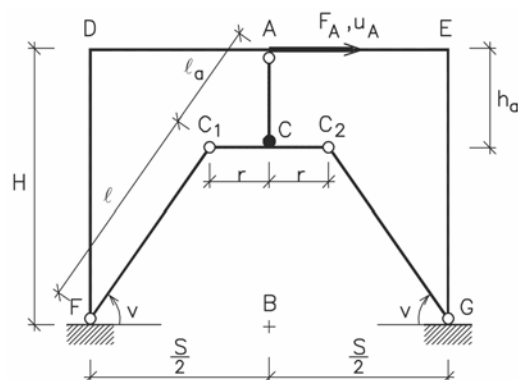
Fig. 2: Frame Upgraded with Friction Damping System
