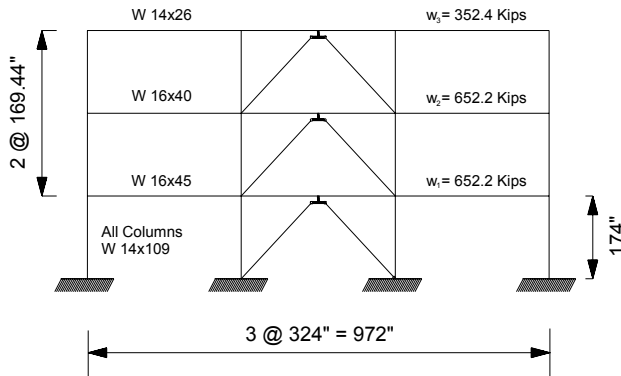
Fig. 6: 3-Story Frame with Damping Device
