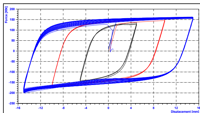
Fig.12. Experimental hysteretic loops at increasing displacements of a buckling restrained axial damper.
